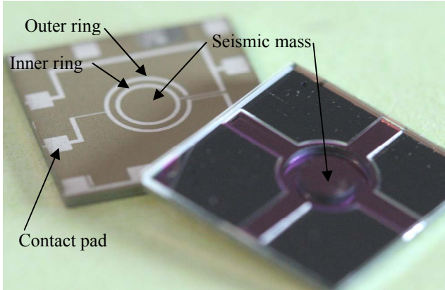
Figure 1. Two 1 cm 2 accelerometer chips seen from the front side (left) and the backside with a bonded pyrex wafer for protection (right).
